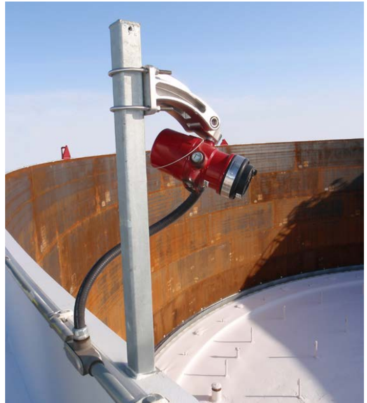
Optical flame detectors can be pole mounted for open-roof internal floating tanks.
